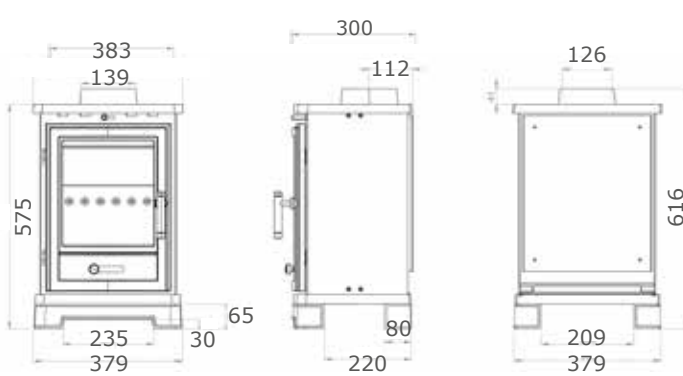
BASSINGTON COMPACT MULTIFUEL BASELINE LEG
